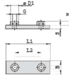
Weld Plate
